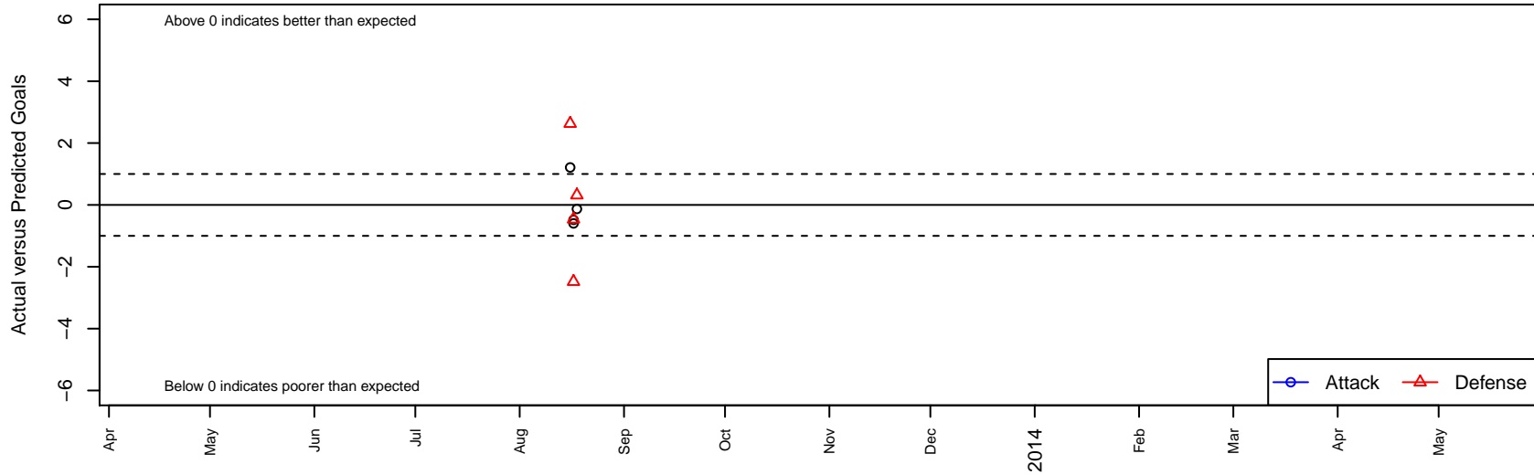
Clackamas Red B02 Dots are actual minus expected GF (blue circles) and GA (red triangles). Blue line is smoothed change in attack strength. Red is smoothed change in defense strength.
